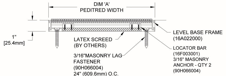
SECTION X-X
